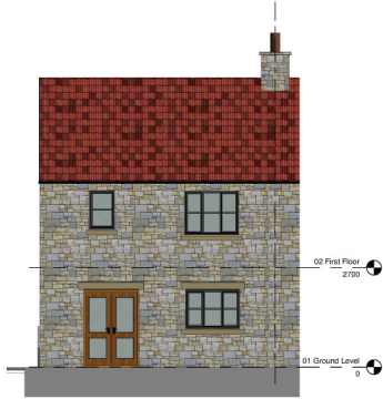
REAR ELEVATION
